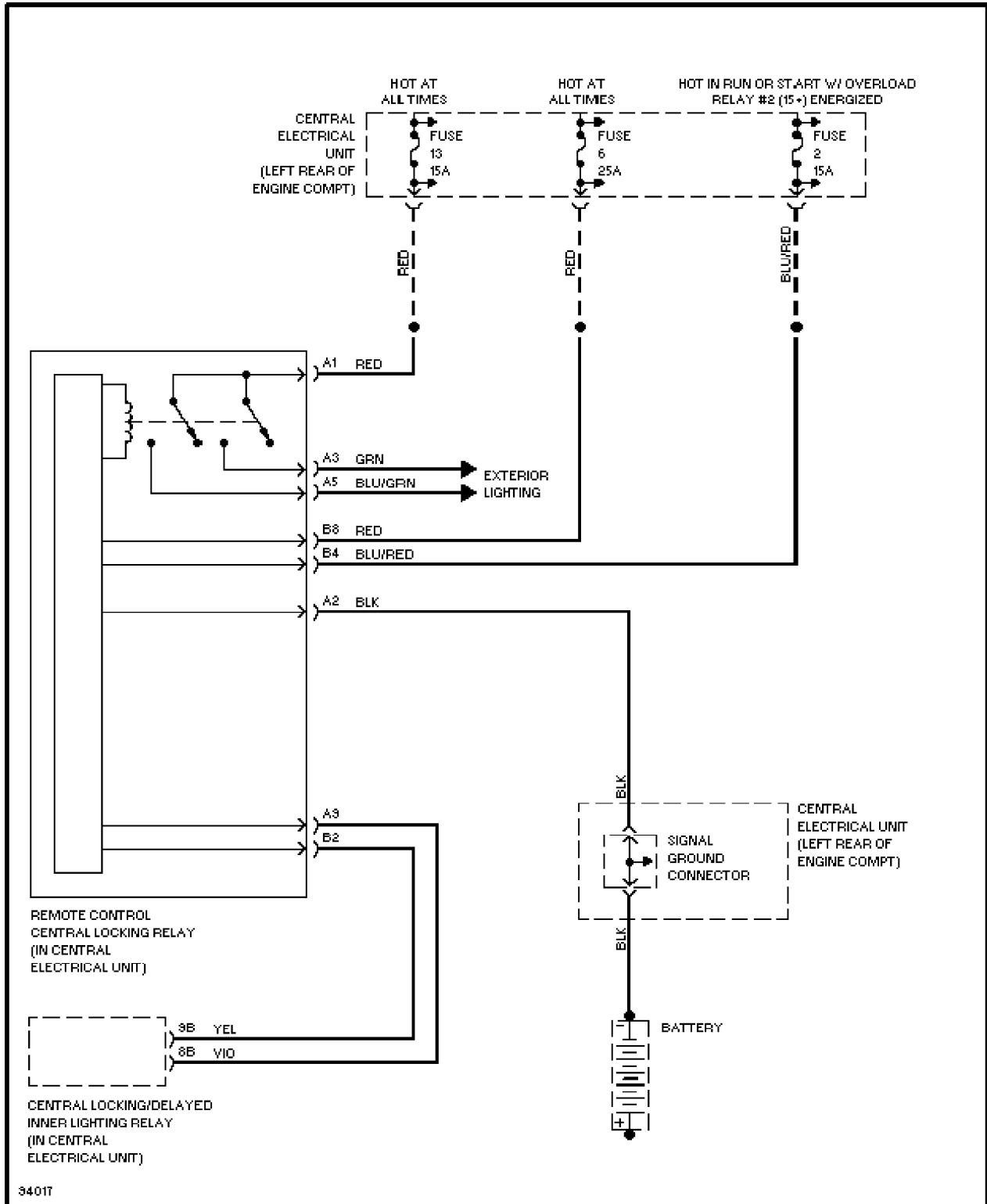
Remote/Central Locking Circuit
