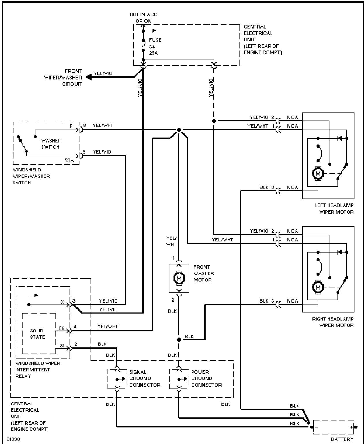
Headlamp Wiper/Washer Circuit
