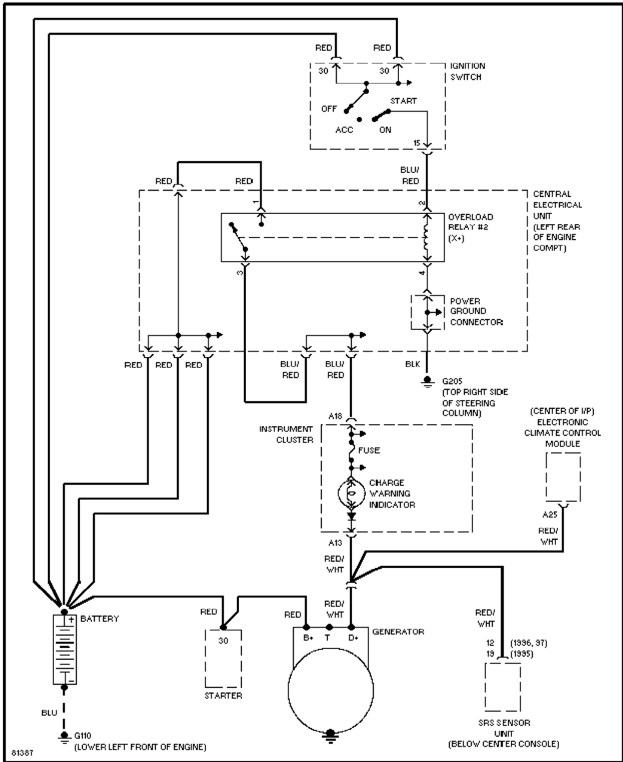
Charging Circuit
