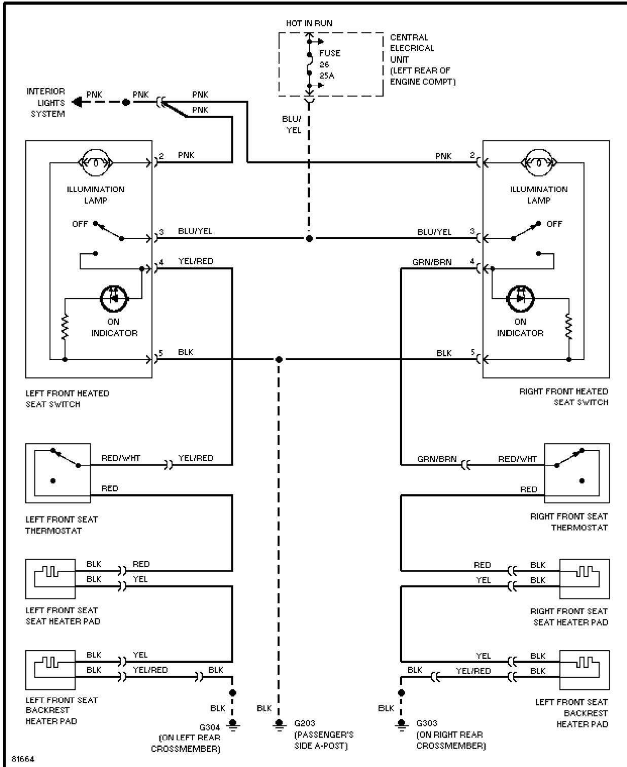
Front Seat Heater Circuit
