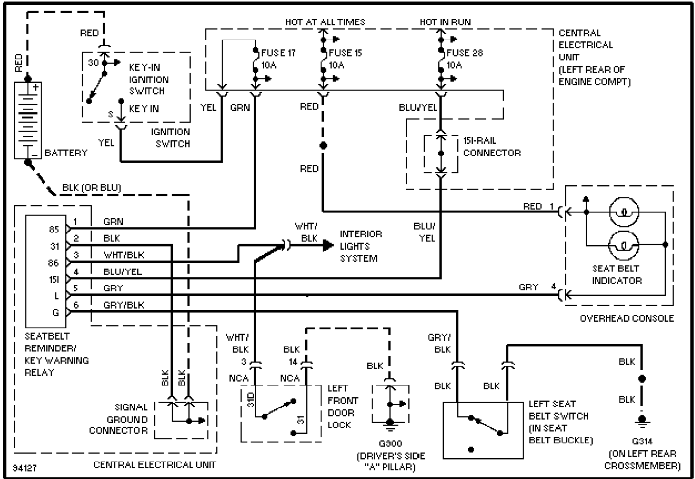
Warning System Circuits
