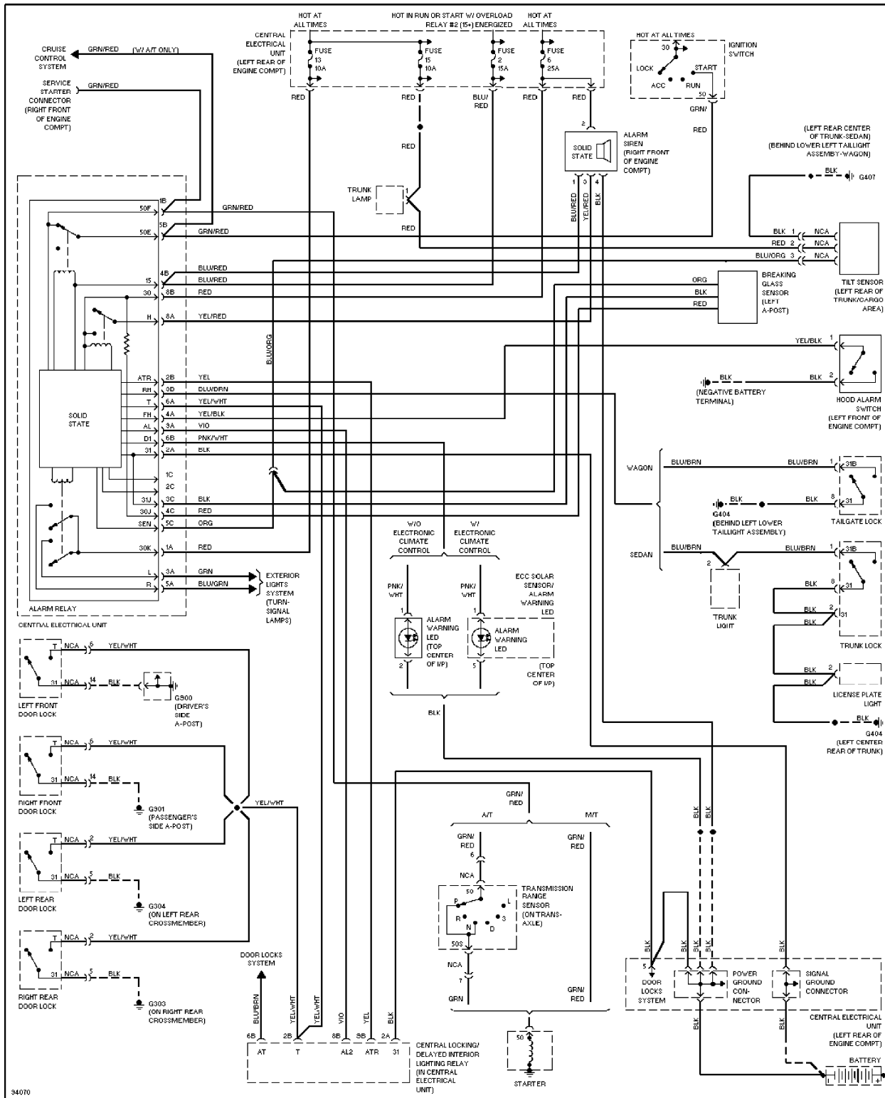
Guard Alarm II Circuit
