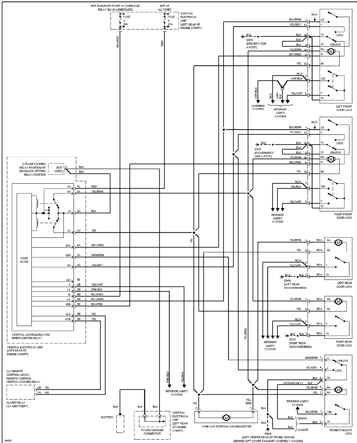
Central Locking Circuit, W/O Deadlock
