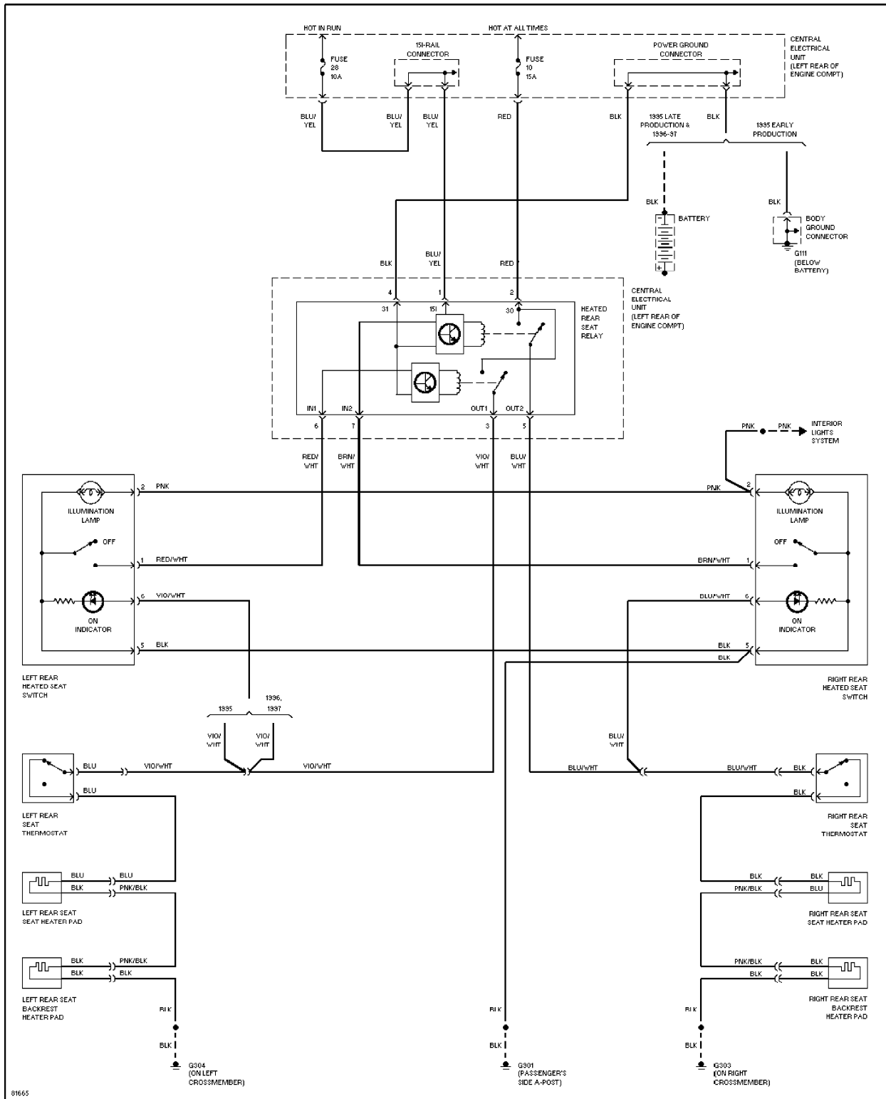
Rear Seat Heater Circuit
