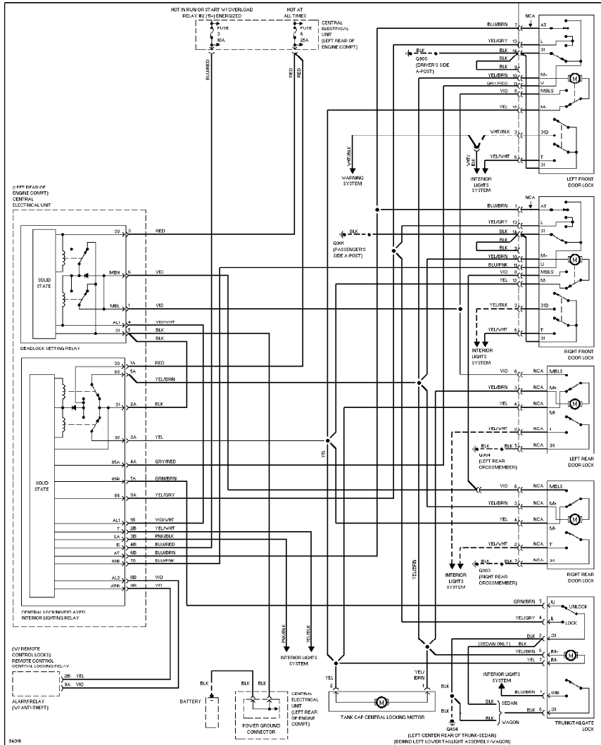
Central Locking Circuit, W/ Deadlock
