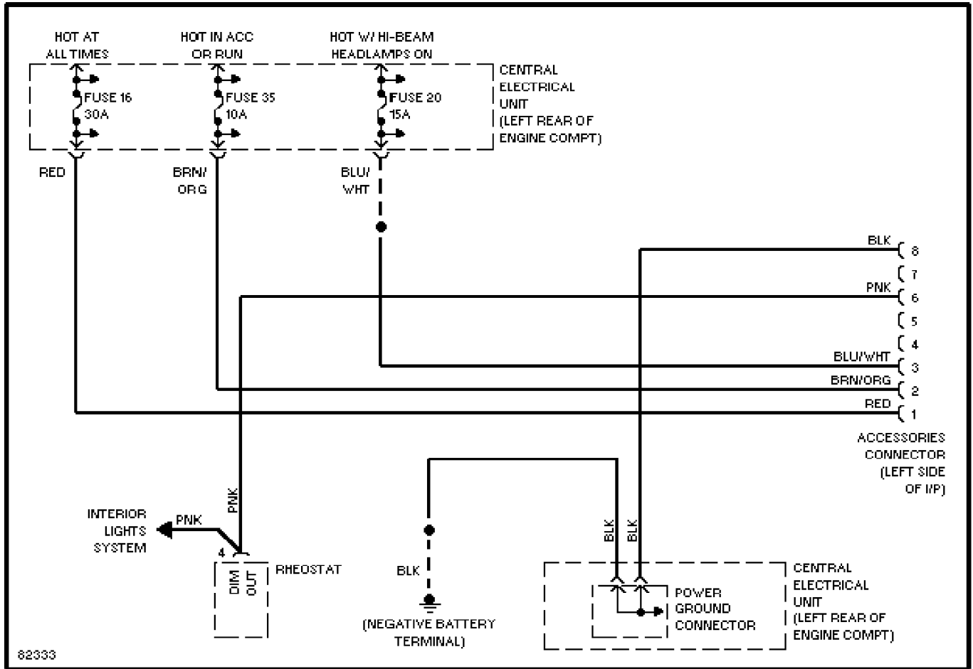
Accessories Connector Circuit
