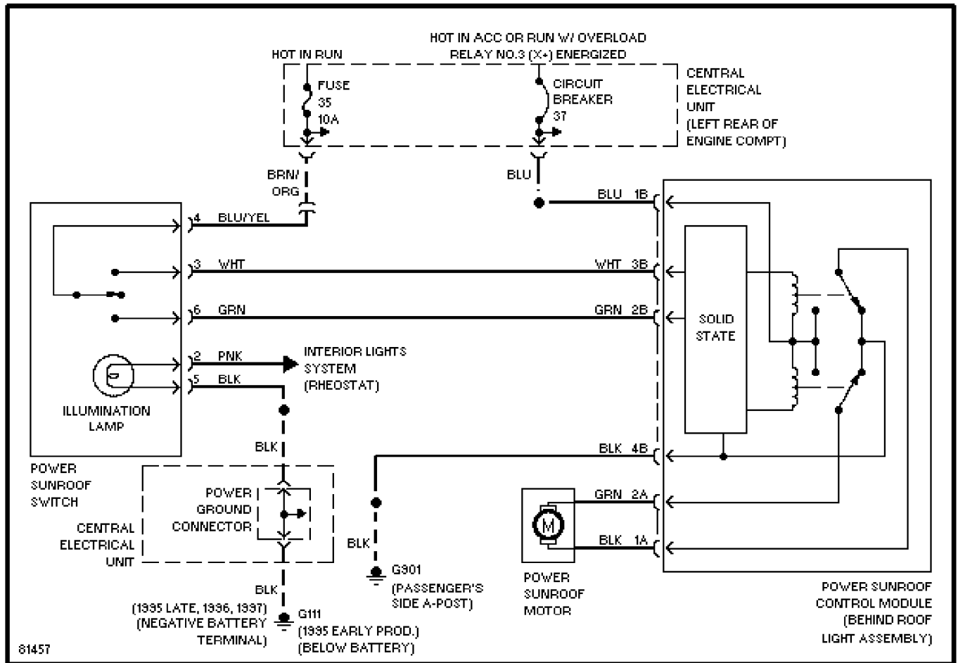
Power Top/Sunroof Circuits
